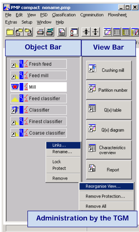
Fig. 1: PMP Table and Graphic Manager for administrating all views within a PMP project
